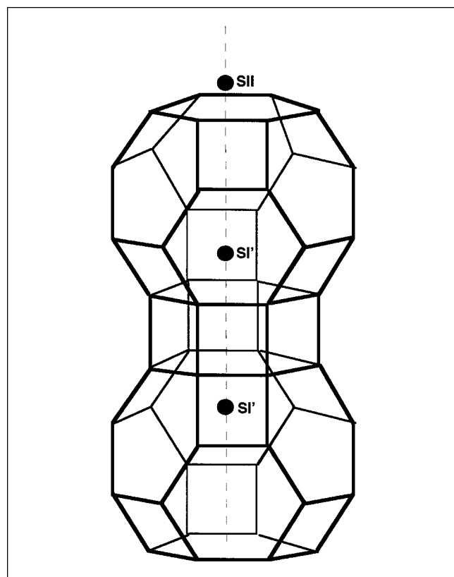
Figure 2. Position of extraframework sites in relation to the sodalite cage in Li–LSX zeolite.
