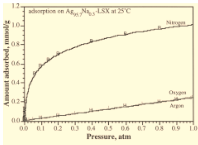
Figure 6. Single-component adsorption isotherms, measured at 25°C, for \text{N}_2 , \text{O}_2 , and Ar on \text{Ag}_{95.7}\text{Na}_{0.3}\text{-LSX} after vacuum dehydration at 450°C for 4 h.
