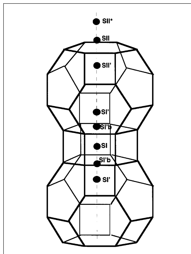
Figure 3. Position of extraframework sites in relation to the sodalite cage in Li,Ag–LSX zeolite.
