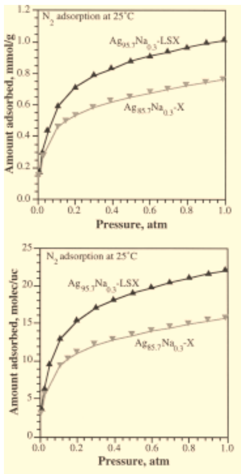
Figure 7. N 2 equilibrium isotherms measured at 25°C.
